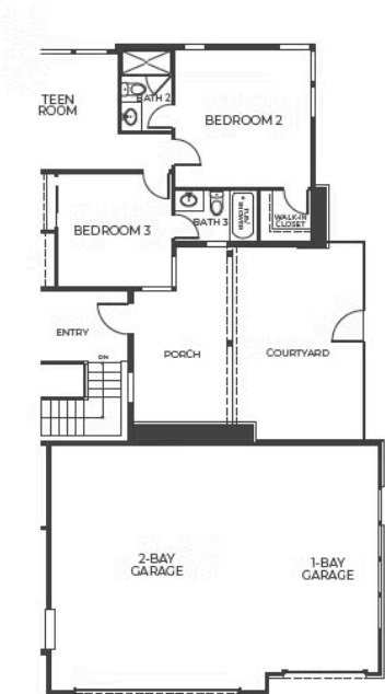
ELEVATION B FIRST FLOOR
